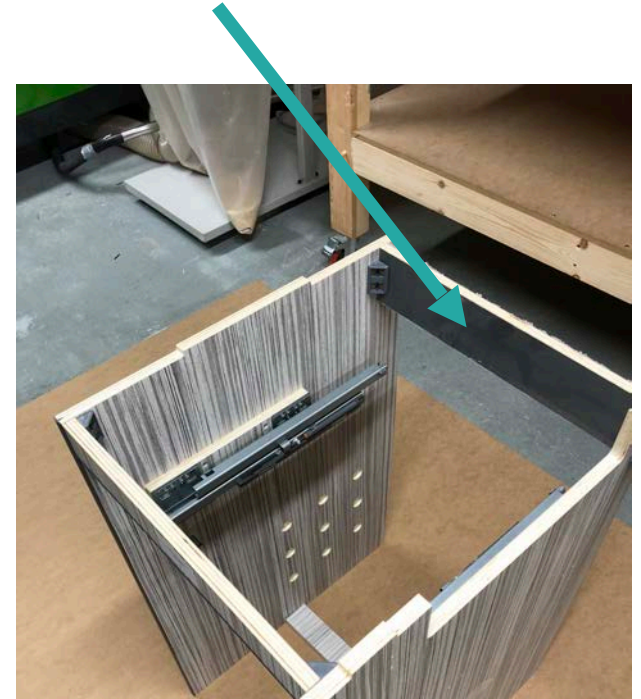
Fit the unit rear support over the finger joint of the fridge pod (R) and chock block to fridge pod upright (L)
