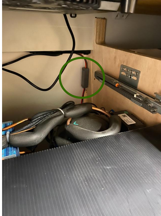
Pull the fridge forward and remove the drawer for wago connection access
