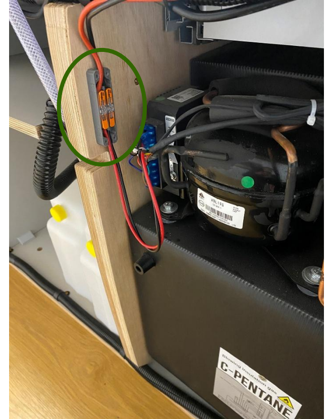
Clip the fridge cables into the wago junction box as per picture and fit cover
